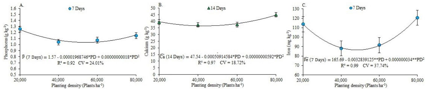
Figure 2. Cladode concentrations of P in the first cycle (A), Ca in the second cycle (B), and Fe in the first cycle (C) for 'Gigante' forage cactus pear as a function of planting density
