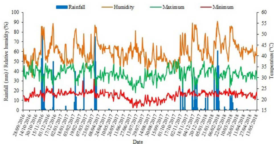
Figure 1. Rainfall, relative air humidity and maximum and minimum temperatures during the experimental period
